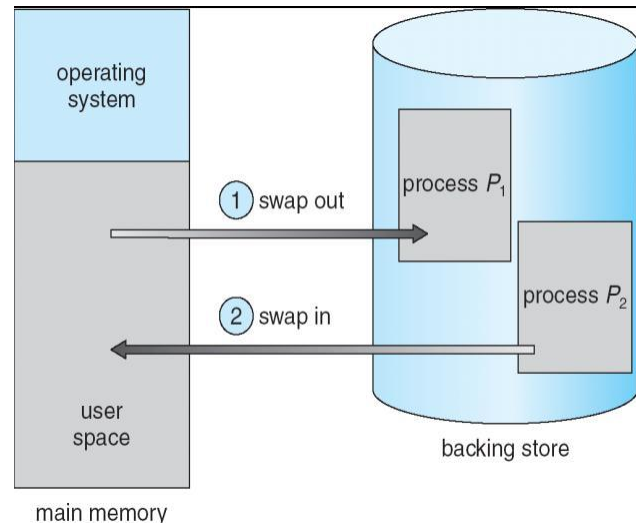
Figure 70: Swapping of two processes using a disk as a backing store
