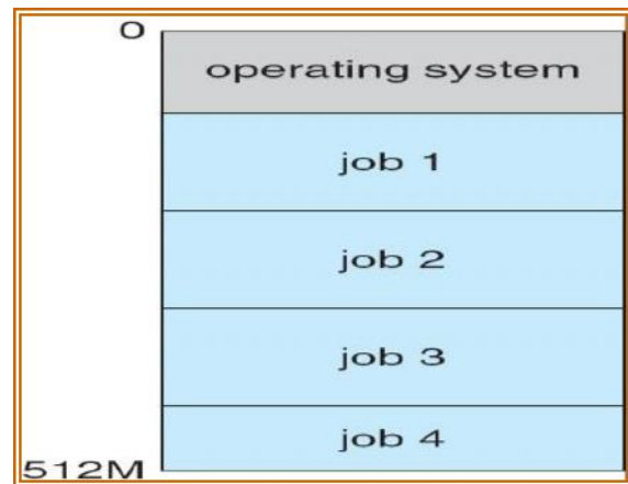
Figure 9: Memory layout for a multiprogramming system
