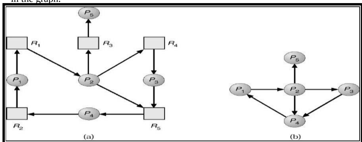
Figure 60: (a): Resource Allocation Graph Fig (b): Corresponding Wait for Graph
