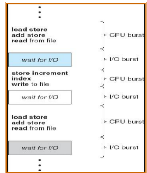
Figure 43: Alternating Sequence of CPU and I/O bursts
