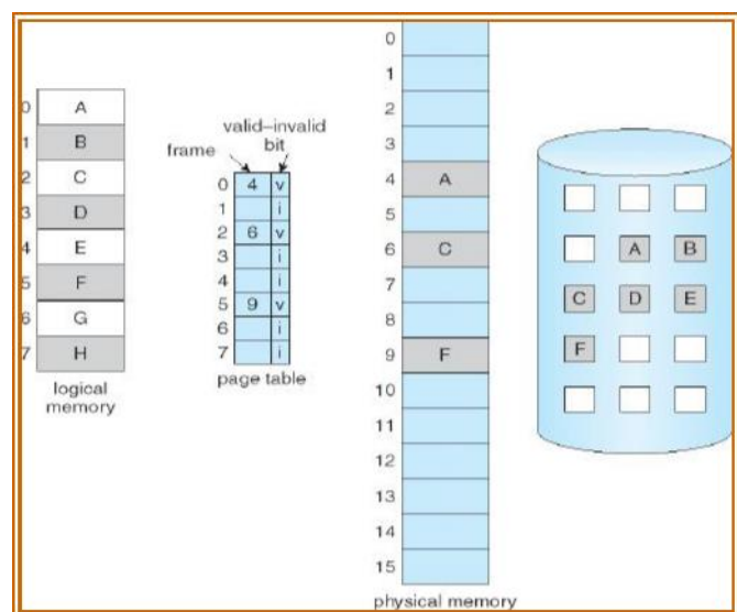
Figure 84: The Picture When All Pages Are Not In Memory
