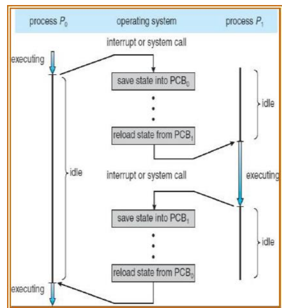
Figure 29: CPU switching between processes
