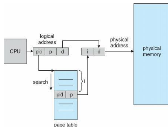
Figure 78: Inverted Page Table
