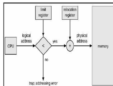
Figure 64: Memory protection using relocation register
