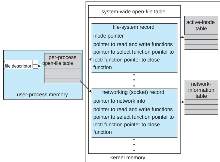
Figure 100: UNIX I/O Kernel Structure
