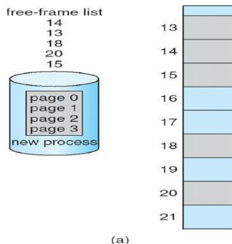
Figure 74: a) Before allocation
