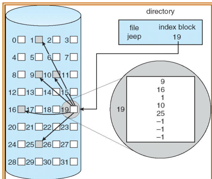
Figure 126: Index Allocation
