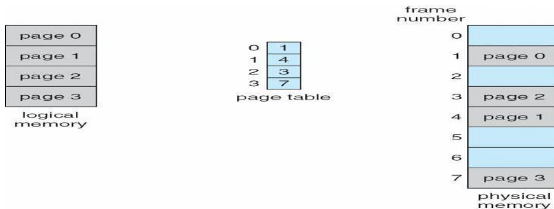
Figure 72: Paging Model
