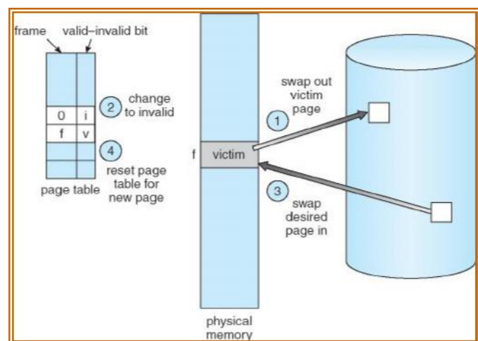
Figure 86: Page replacement
