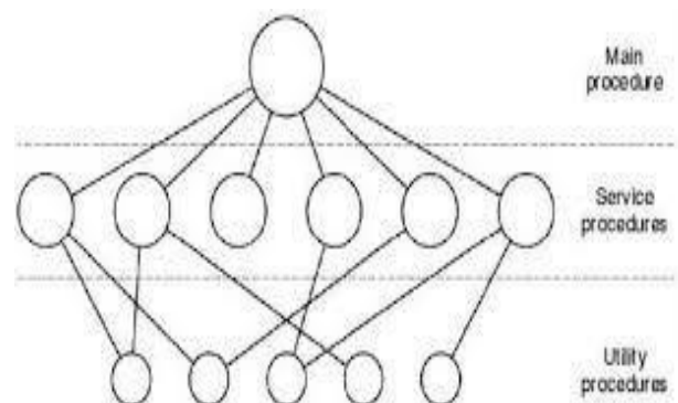
Figure 18: Monolithic structure
