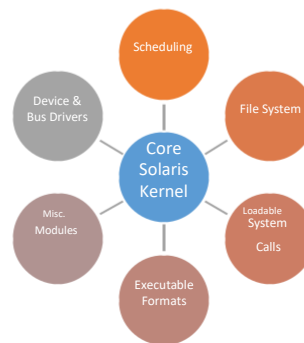
Figure 25: Modules Structure
