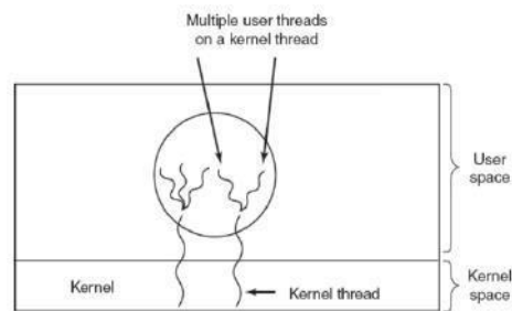
Figure 39: Hybrid Thread
