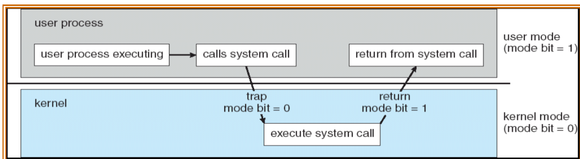
Figure 6: Transition from user mode to kernel mode
