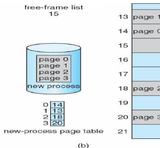
b) After Allocation
