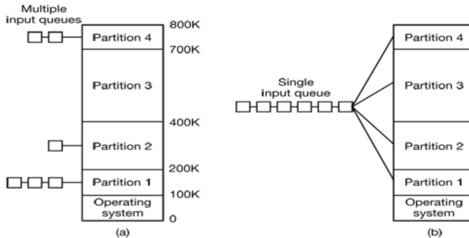
Figure 66: (a) Fixed memory partitions with separate input queues for each partition. (b) Fixed memory partitions with a single input queue
