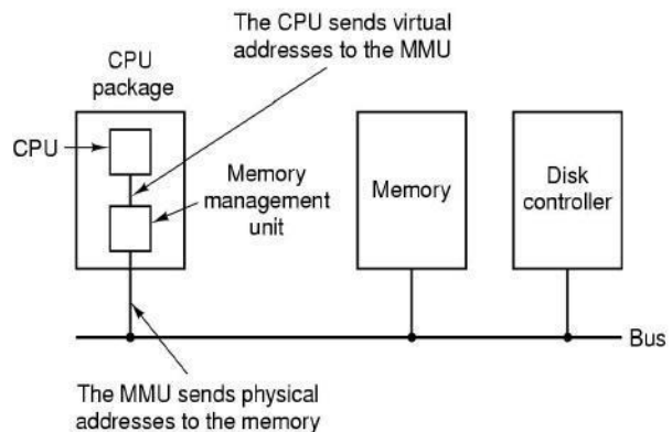
Figure 62: Memory management Unit
