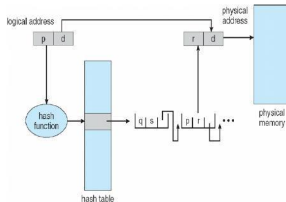
Figure 77: Hashed Page Tables
