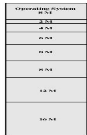
(b) Unequal-size partitions
