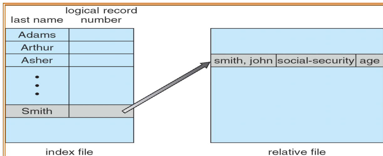
Figure 115: Example of Index and Relative Files
