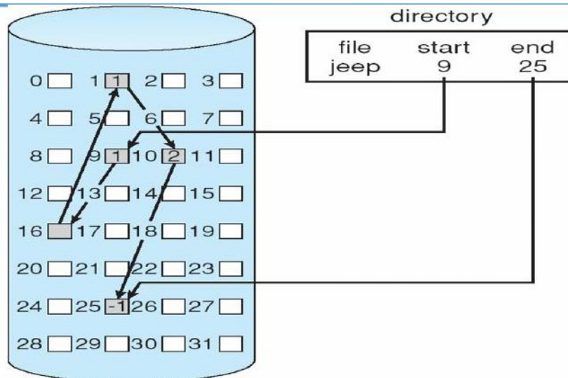
Figure 124: Linked Allocation
