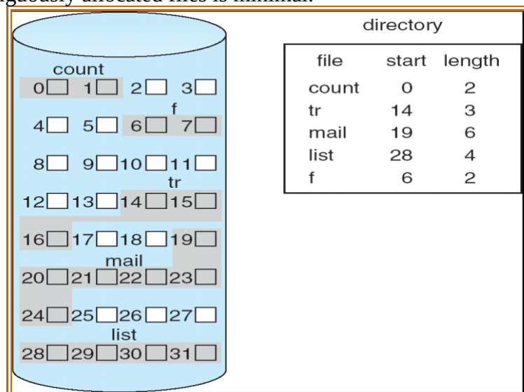
Figure 123: Contiguous Allocation
