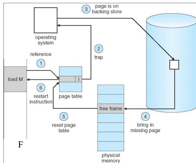
Figure 85: The Picture When All Pages Are Not In Memory
