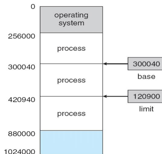
Figure 61: A base and limit register define a logical address space.
