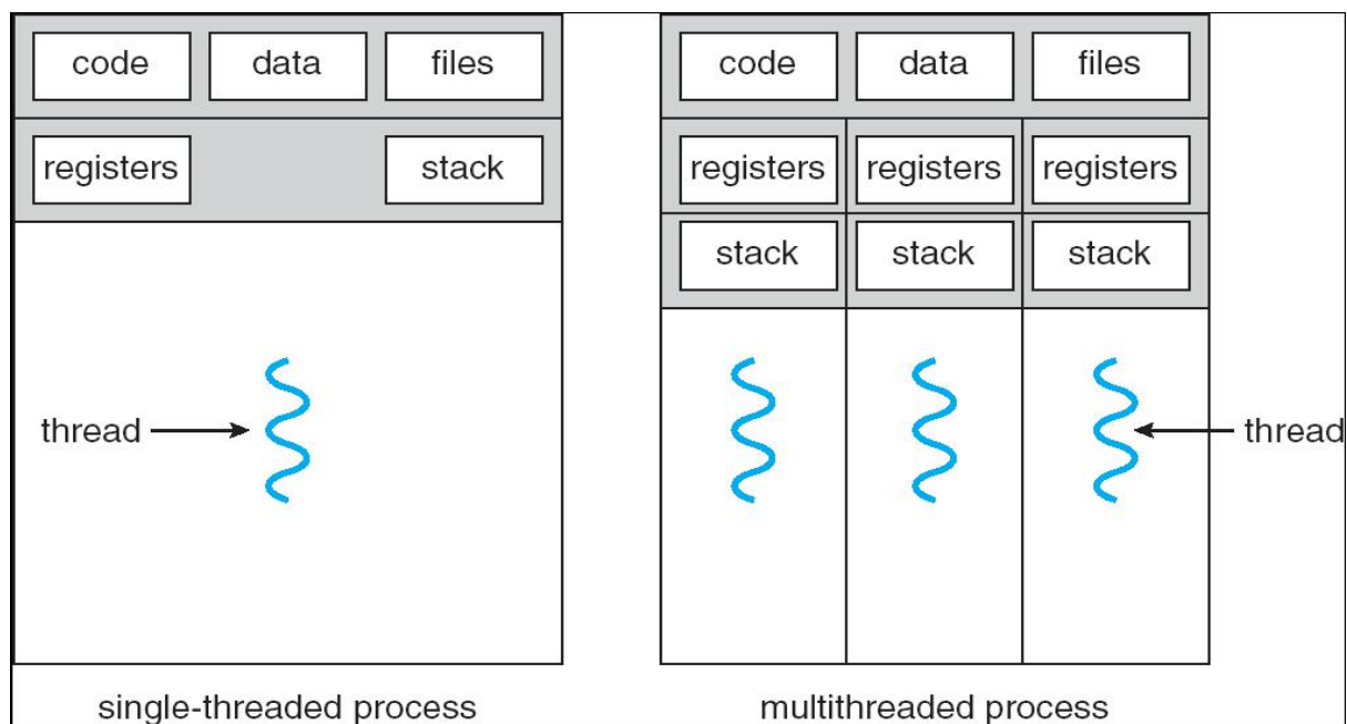
Figure 34: Single and multithreaded process.
