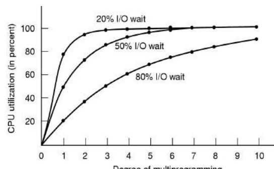
Fig: CPU utilization as a function of number of processes in memory
