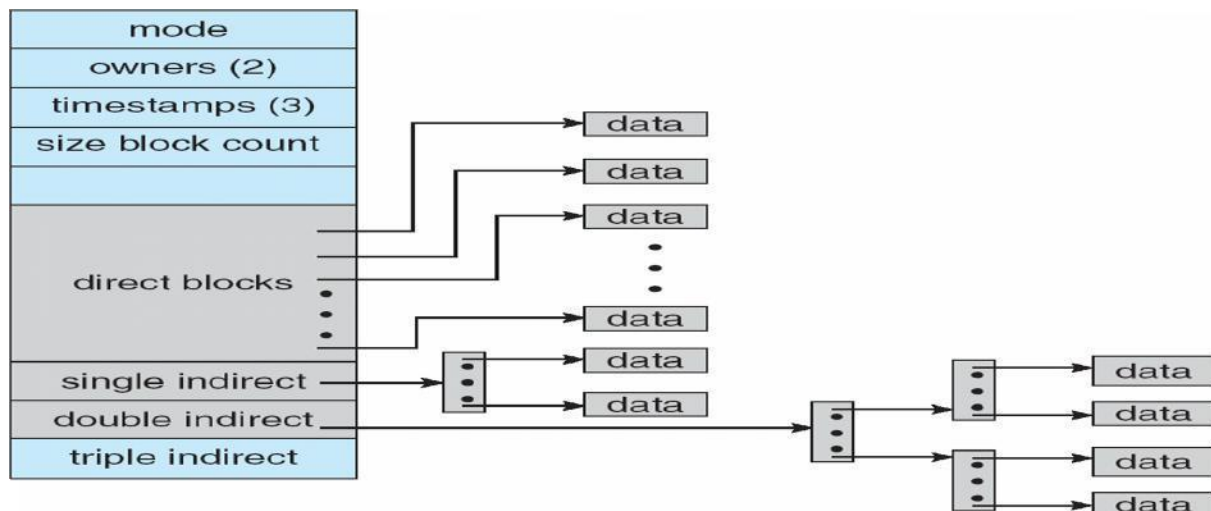
Figure 128: Combined Scheme: UNIX UFS
