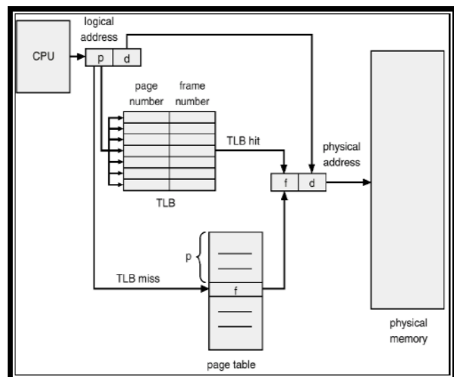
Figure 76: Paging Hardware with TLB
